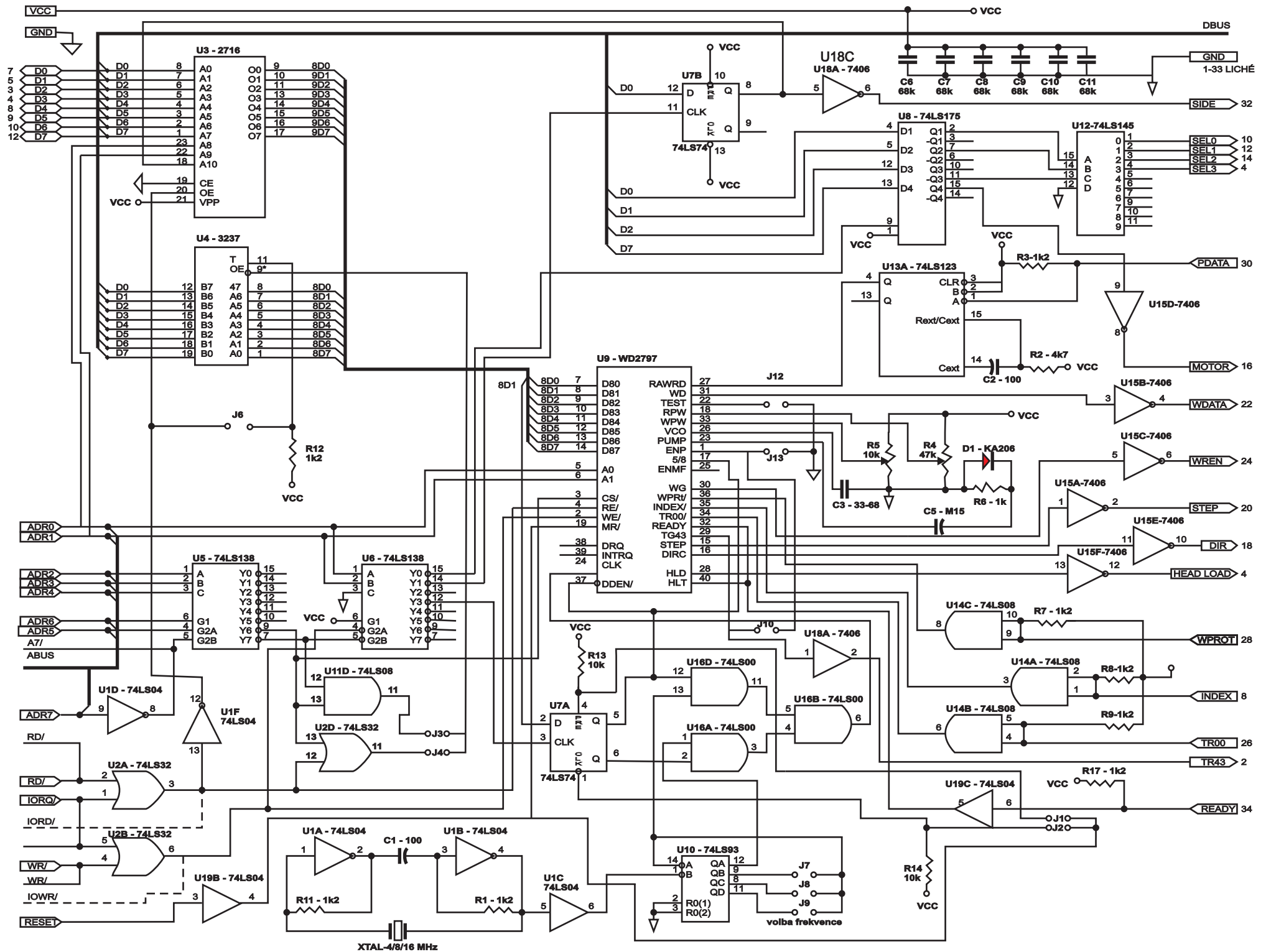
XTAL-4/8/16 MHz
